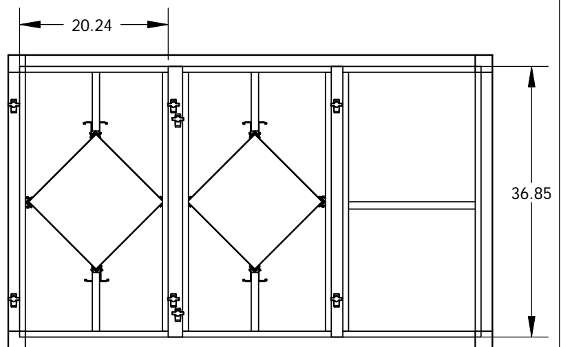
TOP VIEW (ACCESS PANELS REMOVED)
